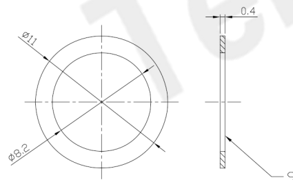
Washer
