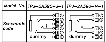
□:Terminal No. ○:Item No. Circuit Diagram
