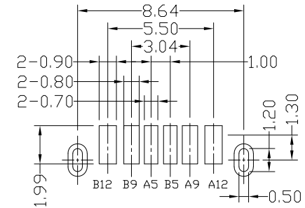
RECOMMENDED P.C.B. LAYOUT TOLERANCE UNSPECIFIED ±0.05mm
