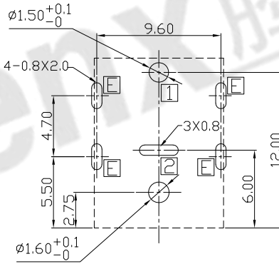
RECOMMENDED P.C.B. LAYOUT UNSPECIFIED TOLERANCE: ±0.05 (TOP VIEW)
